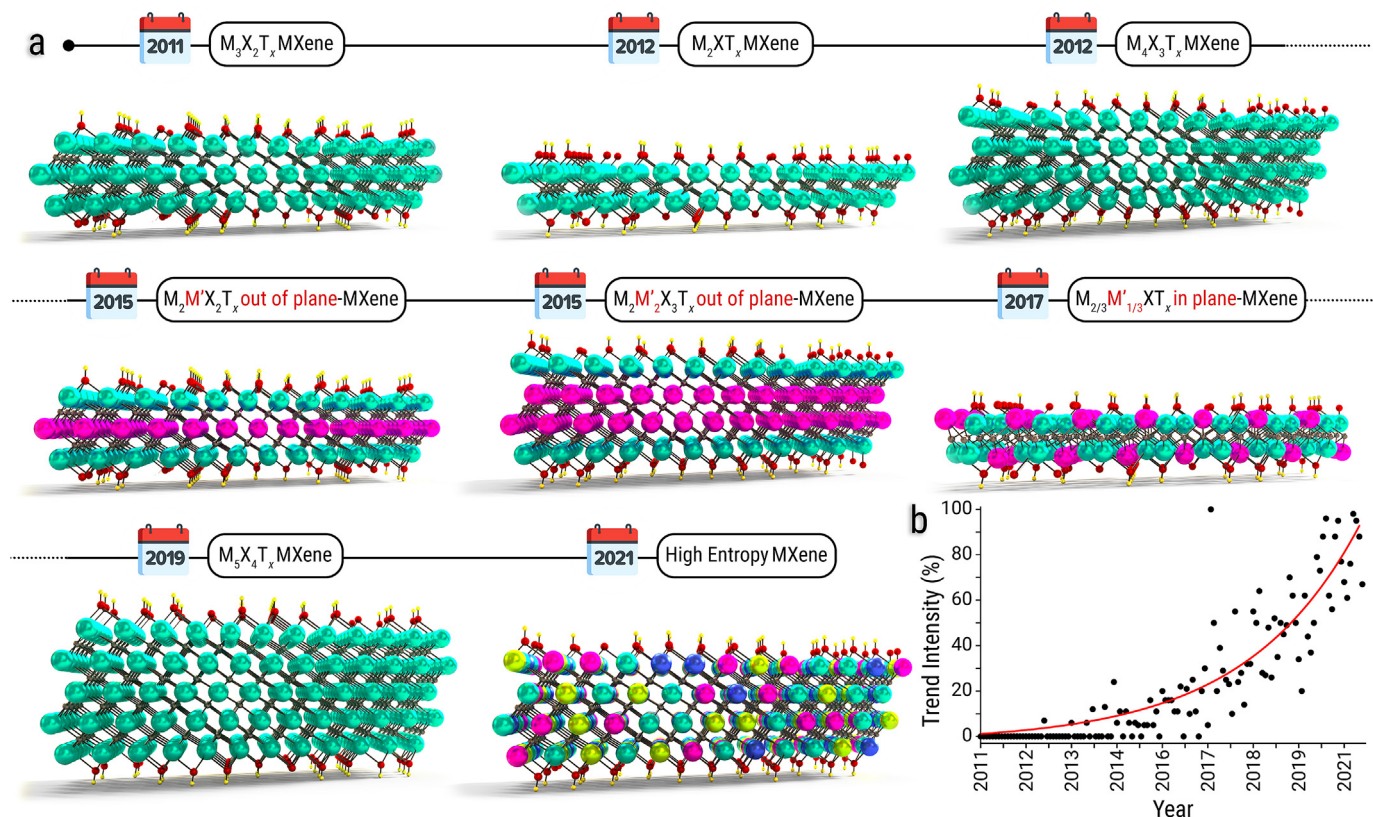
Fig. 1. (a) The schematic illustration of different MXene structures. Ti_3C_2T_x , as an example of M_3X_2T_x MXene (top left), was the first discovered MXene in 2011, followed by the discovery of M_2XT_x and M_4X_3T_x in 2012. The family of MXenes was expanded by the addition of ordered double-transition metal MXenes, out-of-plane ordered in 2015 followed by in-plane ordered in 2017. M_5X_4T_x solid solution MXene and high-entropy M_4X_3T_x MXenes are among the latest additions to the MXenes family. The green, yellow, pink, and blue color spheres represent early transition metals in MXenes. Surface terminations of MXenes are randomly scattered and attached to the outer atomic layer of the MXene structure, which are mainly O, F, or OH groups. (b) The monthly Google Trends data, collected over the decade from users' engagement with the word "MXene." These data are proportional, and the highest value is normalized to 100. Since 2015, there has been a considerable increase in trend intensity. Google Trends data in this work were mined using the "pytrends" Python library [8].
